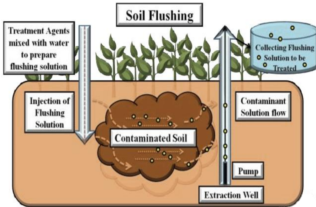
Figure 5.2. Soil flushing process (Ramanlal & al. 2022)
