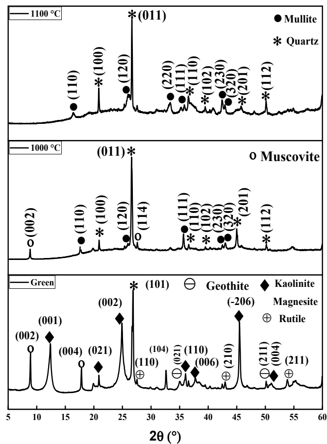
Figure 5. XRD patterns of K94M6 (green tapes and tapes sintered at 1000 and 1100 ^{\circ}\text{C} ).
