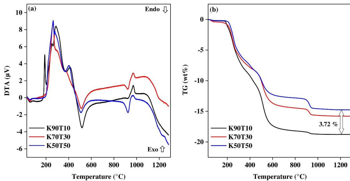
Figure 4. DTA (a) and TG (b) curves of three kaolin-talc tapes (under air up to 1200 ^{\circ}\text{C} ), K50T50, K70T30, and K90T10.
