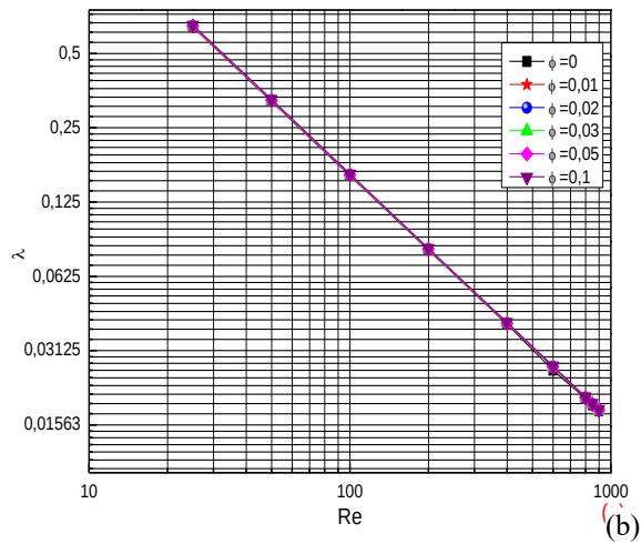
Figure 5. Skin friction coefficient versus: (a) volume fraction of \text{SiO}_2 nanoparticles and (b) Reynolds numbers
