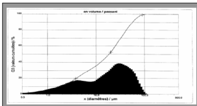
Fig. 1. Size distribution of cement CEM I 52.5
